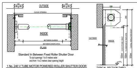
1 No. 240 V TUBE MOTOR POWERED ROLLER SHUTTER DOOR
